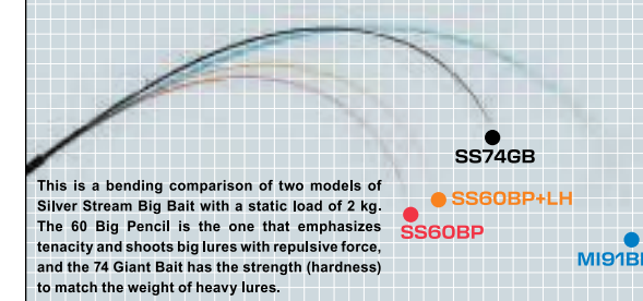
SilverStream BIG BAIT Bending Curve Load 2kg Static load comparison
