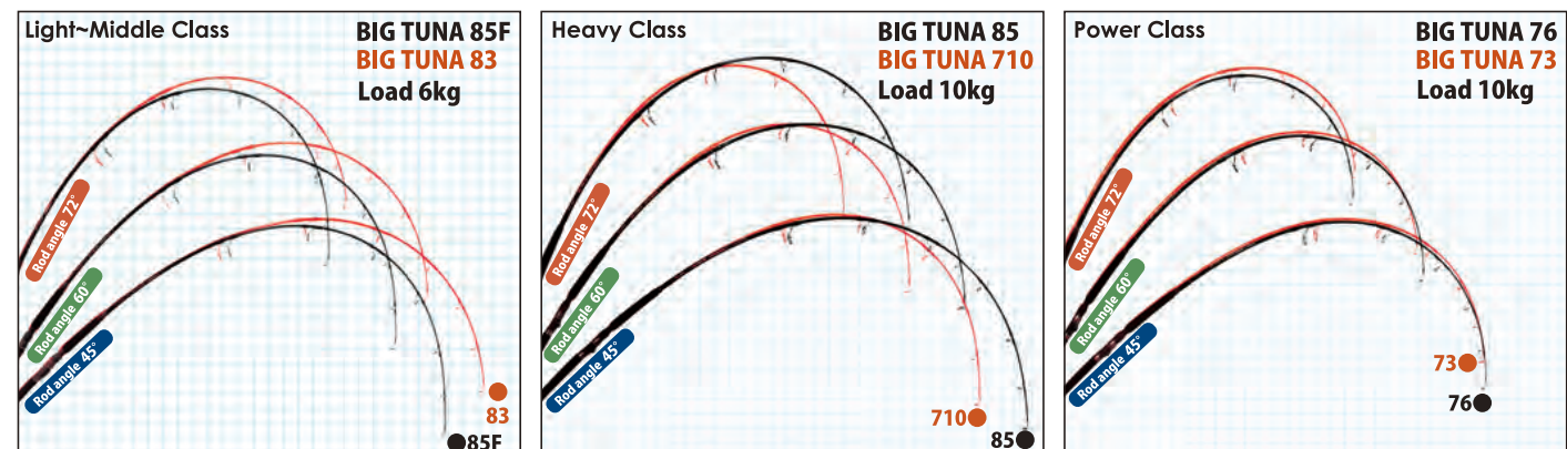
Static load comparison of BIG TUNA 85F & BIG TUNA 83 (6kg load) Static load comparison of BIG TUNA 85 & BIG TUNA 710 (10kg load) Static load comparison of BIG TUNA 76 and BIG TUNA 73 (10kg load)
